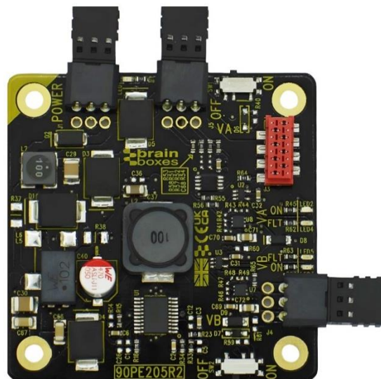
Figure 1 – PE-205 Embedded Power Supply Module
